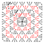
Schema 1: granny
